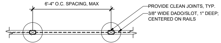
PLAN
