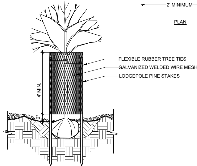
SECTION
