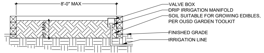
SECTION ELEVATION
